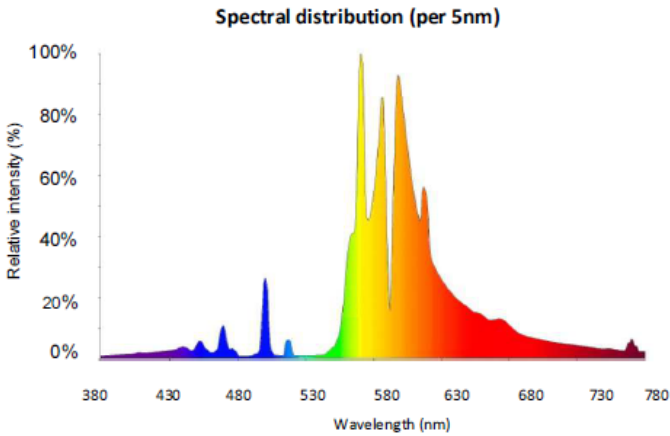
Spectral Power Distribution Color - MASTER GreenPower Xtra 1000W EL II UNP/50
